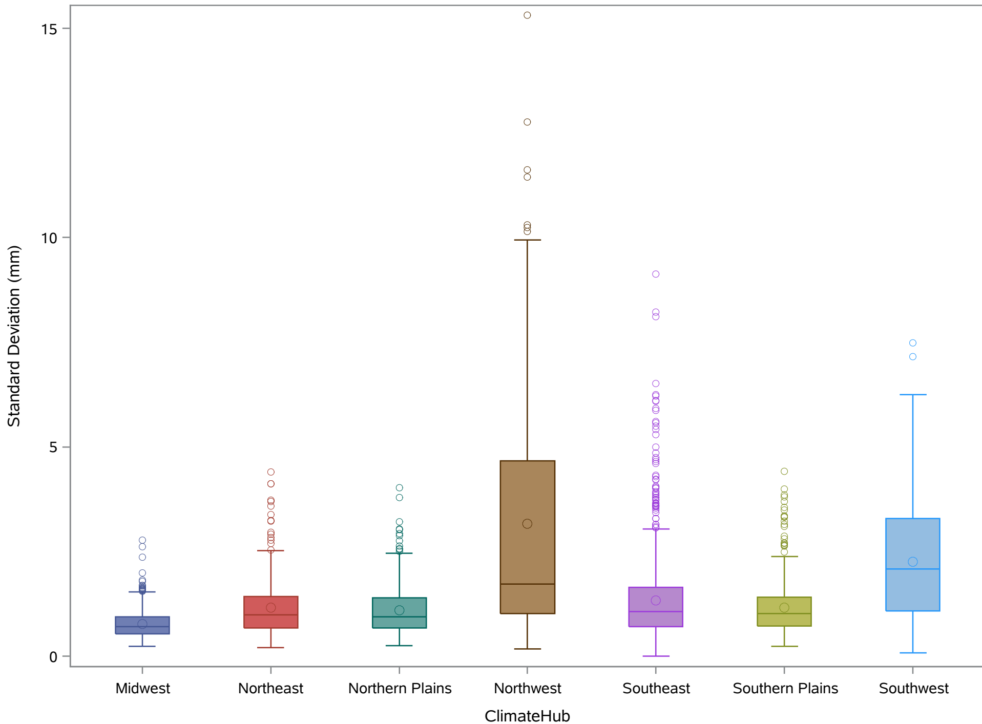
Standard Deviation of Summer Precipitation
